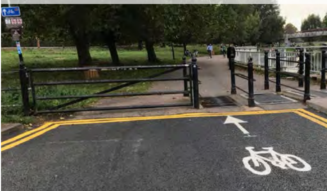
Figure 8.4: Cattle grid access control, Cambridge
