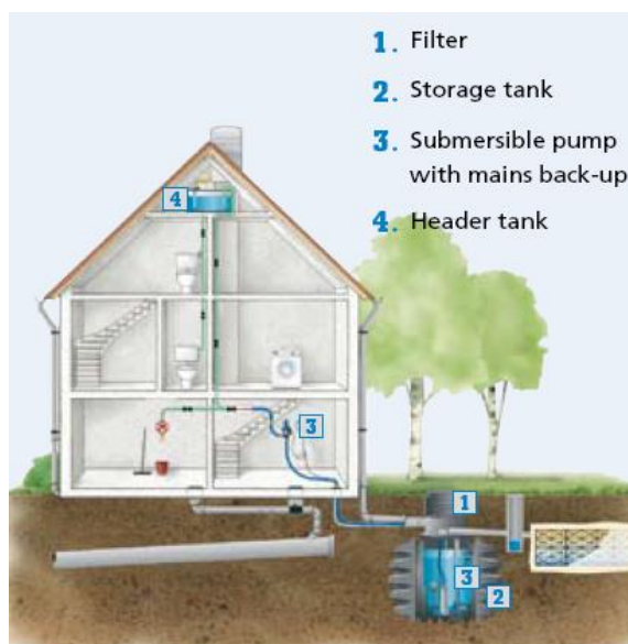
Figure D-1: A typical domestic rainwater harvesting system
